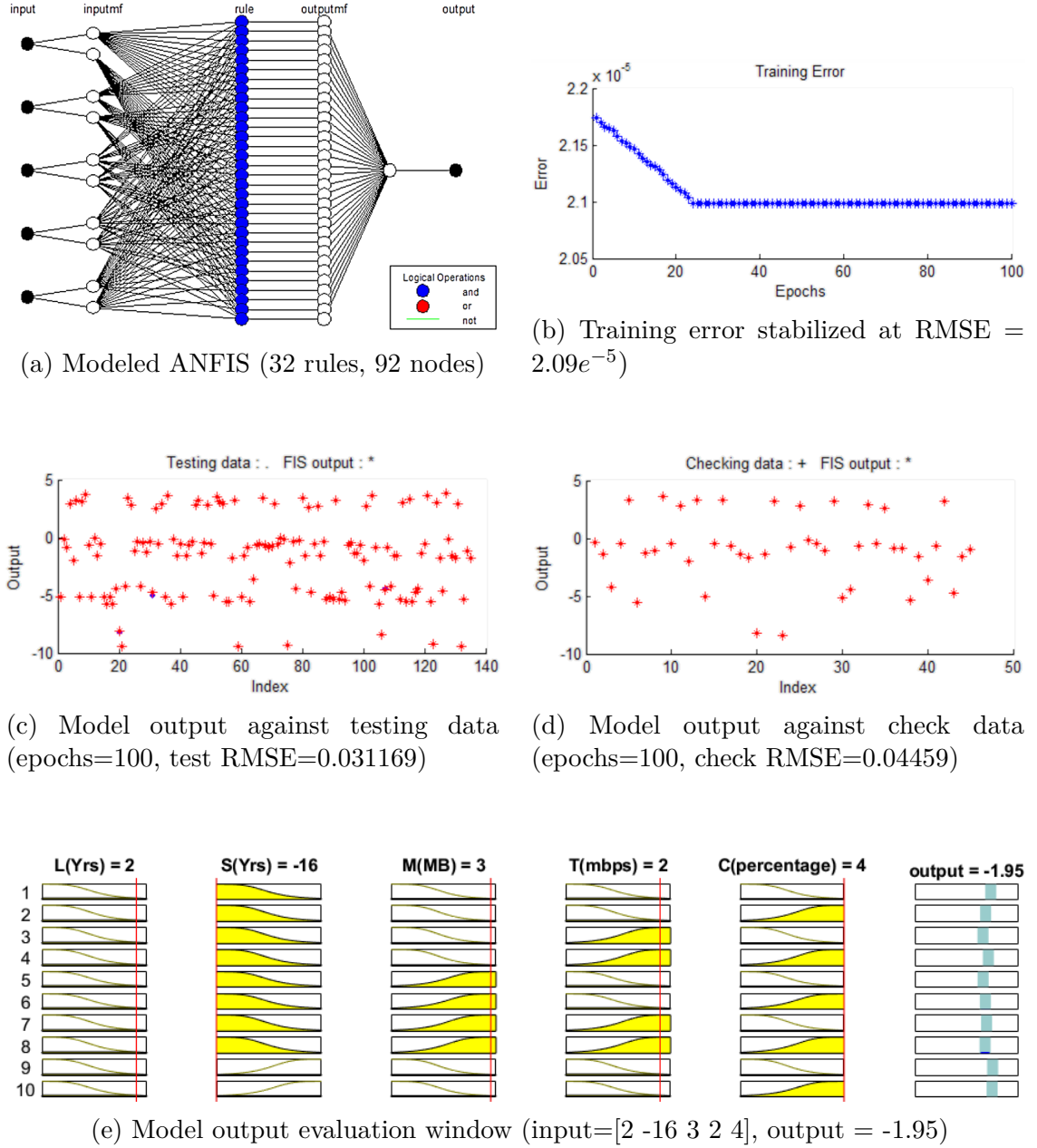
Figure 5.1: Training, testing, and validation results
