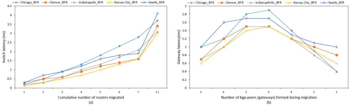
Figure 5.30: Control path latency with BFR in Abilene Network, while setting Chicago, Denver, Indianapolis, Kansas City, and Seattle as RSS. Control path latency by (a) switch, (b) iBGP-peers formed during migration
