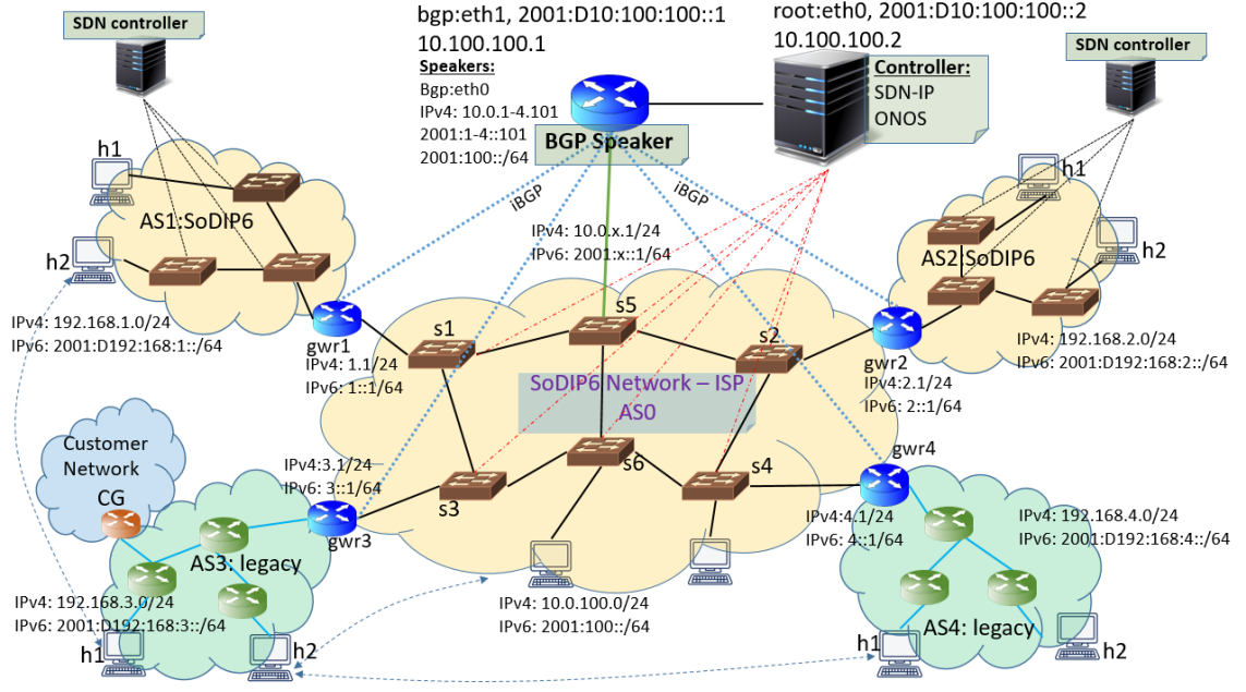
Figure 5.24: Implemented multi-domain SoDIP6 network environment
