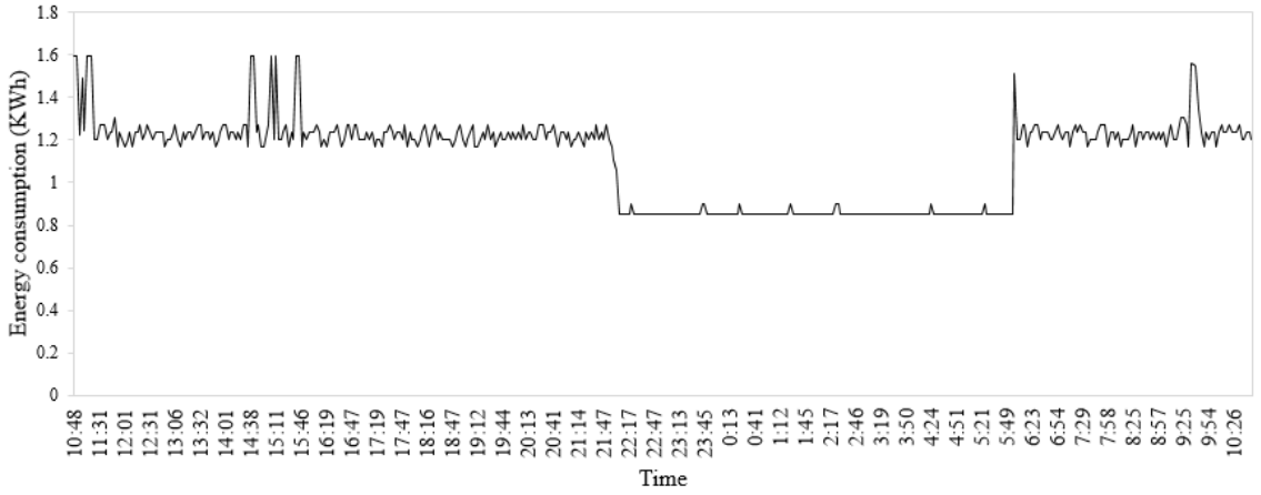
Figure 5.34: Pattern of total energy consumption by SoDIP6 capable switches and CPEs
