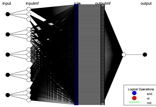
(a) Modeled ANFIS (243 rules, 524 nodes)
