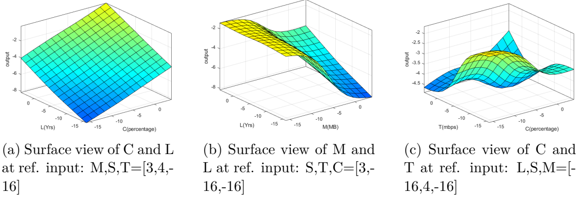
Figure 5.2: Surface view of input parameters for ANFIS model at different reference inputs
